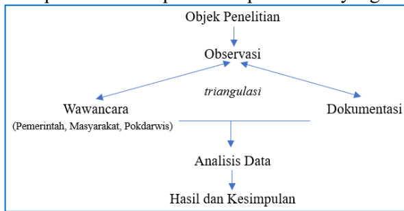
Gambar 3. Alur Penelitian
